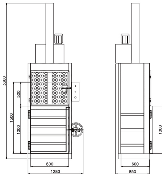
Bale Size ( Model XTY-300KL8060 )
